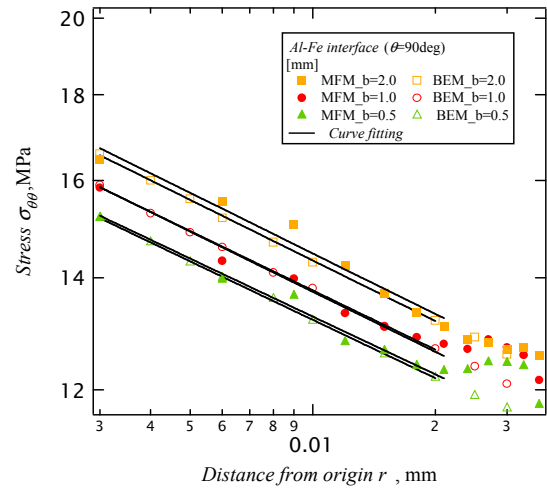
Figure 7. Comparison of stress distribution of \sigma_{\theta\theta} for radius direction from vertex in case of MFM and BEM ( \phi=45\text{deg} \theta=90\text{deg} )
