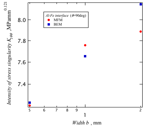
Figure 8. Comparison of intensity of stress singularity with respect to model width “b” in case of MFM and BEM
