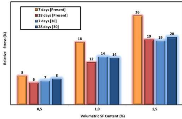
Figure 8: Relative stress – SF content (%) evolutions.
