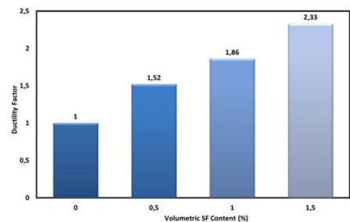
Figure 14: Ductility factor.
