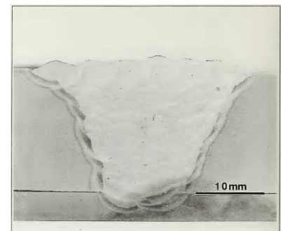
Welded at 31 o C water temperature and 7.3 m water depth
