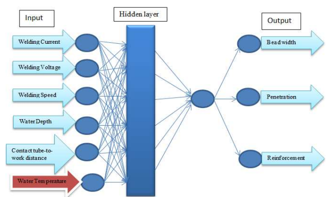
Fig. 1. Welding input vs output parameters.
