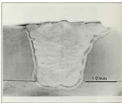
Welded at 2.8 o C water temperature and 6.7 m water depth
