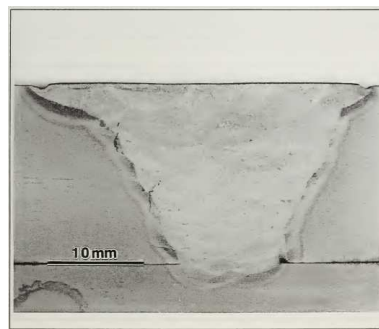
Welded at 10 o C water temperature and 5.5 m water depth
