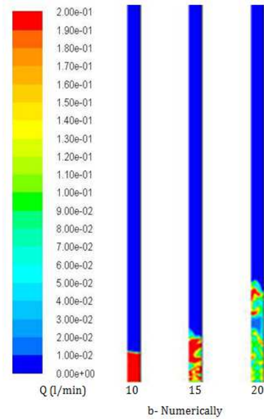
Fig. 5. Flow behavior at 2.5 cm H and different values of water flow rate.
