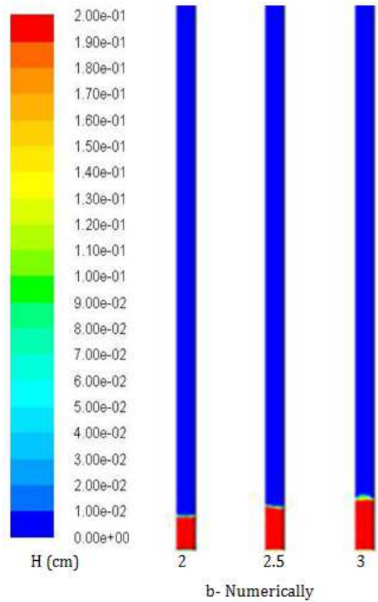
Fig. 7. Flow behavior at 10 l/min water flow rate and different values of H.
