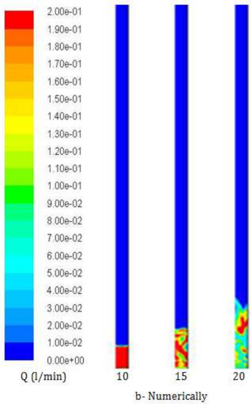
Fig. 4. Flow behavior at 2 cm H and different values of water flow rate.
