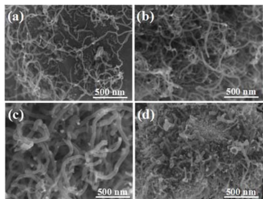
Figure 4. SEM images: (a) CNTs/SiCp(2.5 wt.% Ni), (b) CNTs/SiCp(5.0 wt.% Ni), (c) CNTs/SiCp(7.5 wt.% Ni), (d) CNTs/SiCp(10.0 wt.% Ni).
