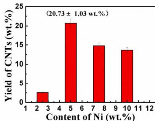
Figure 3. Yield of CNTs with different content of Ni catalyst.
