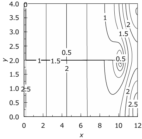
Figure 5. Pressure ( p ) distribution in base case.
